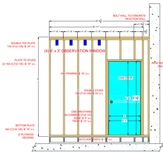
Figure 1. Wall Interior/Gypsum Side
