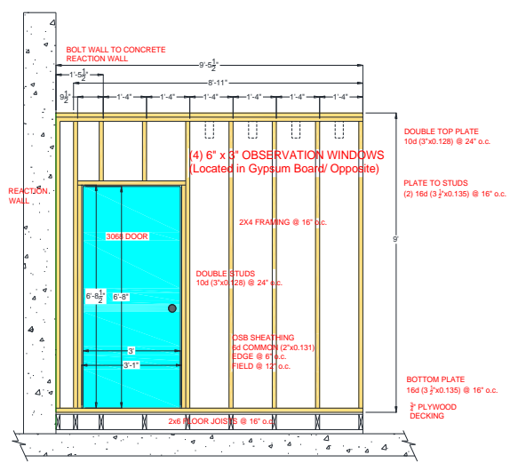
Figure 2. Wall Exterior/OSB Side
