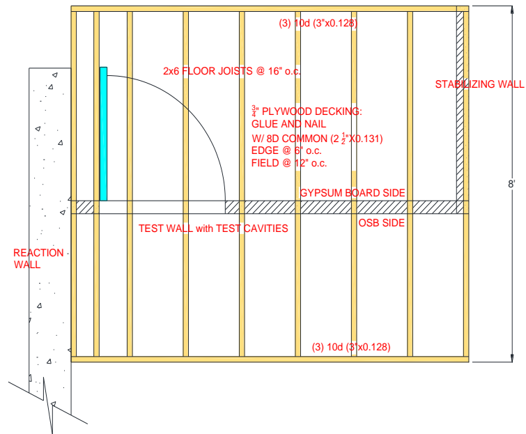
Figure 3. Plan View
