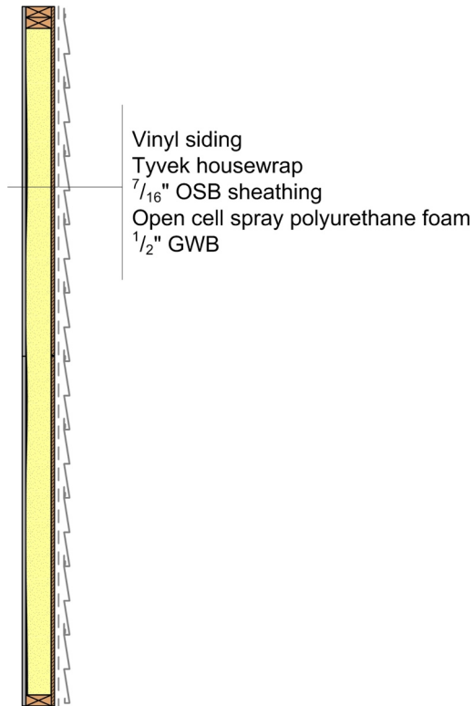
Figure 65: Vertical Section for Reference Wall 5 - ocSPF
