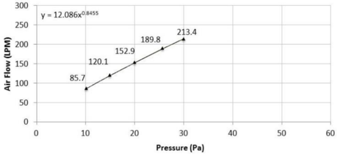
Wall 4- 2x4 ds-CFI: Air Flow Testing
