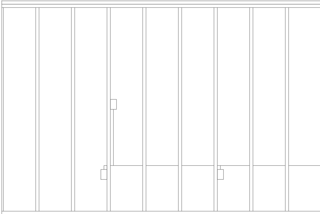
Figure 68 – Elevation of Framing & Electrical for Reference Wall 6 – ccSPF
