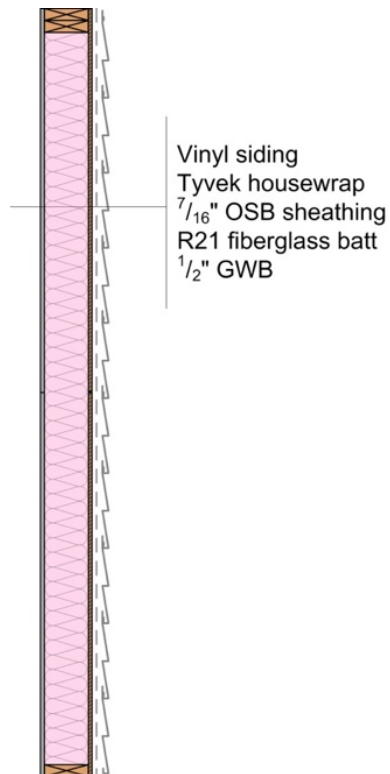
Figure 73 – Vertical Section for Reference Wall 8 – 2x6 F.G. Batt
