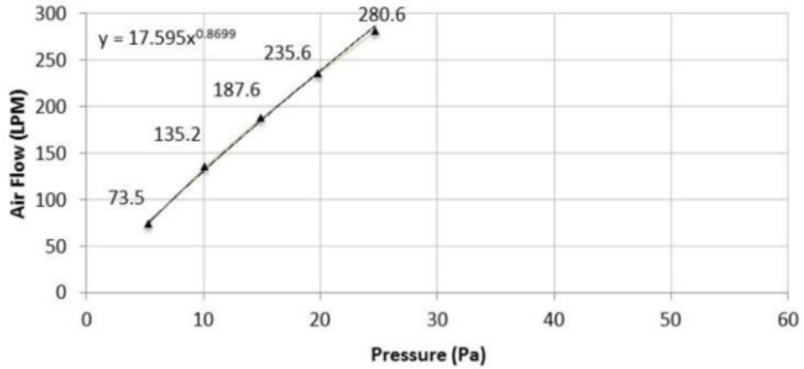
Wall 3- 2x4 Inset-Stapled F.G. Batt: Air Flow Testing
