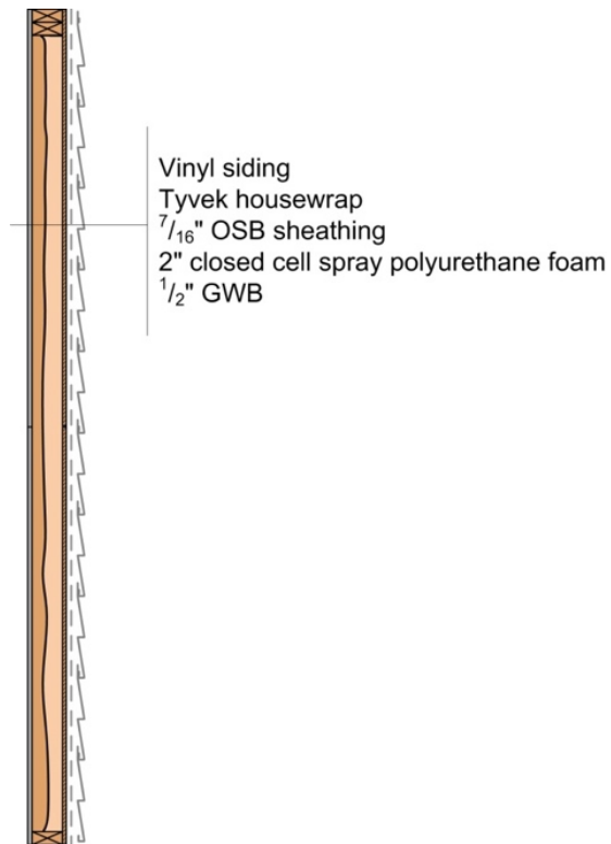
Figure 69 – Vertical Section for Reference Wall 6 - ccSPF
