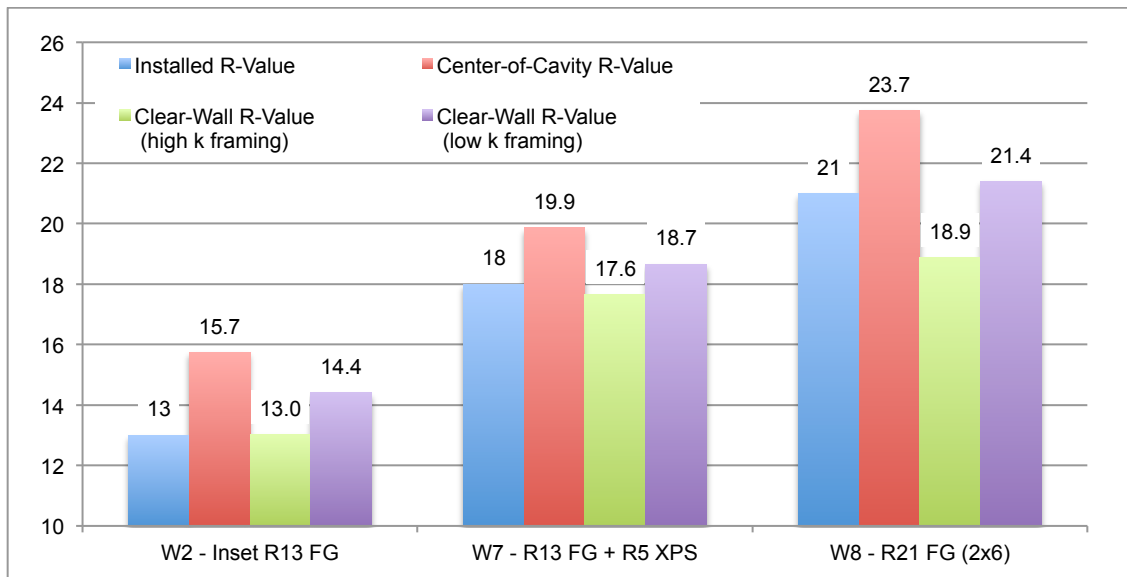
Figure ES-1 – Common Thermal Metrics for Reference Walls 2, 7, and 8
