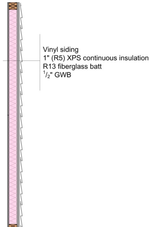
Figure 71 – Vertical Section for Reference Wall 7 – 2x4 F.G. Batt with 1” XPS
