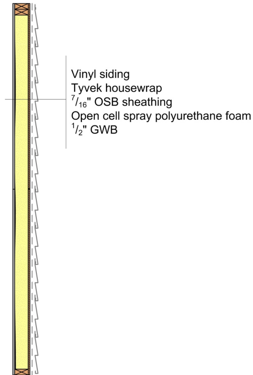
Figure 67: Vertical Section for Reference Wall 5 II - ocSPF
