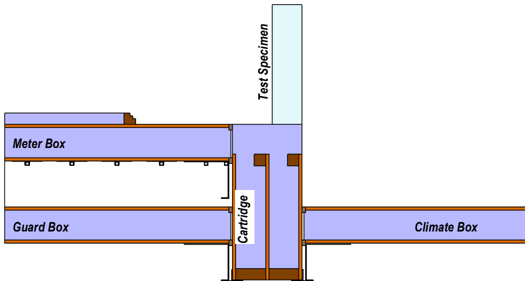
Figure 7 – Section through Wall Cartridge with Meter, Guard and Climate Boxes in Position
