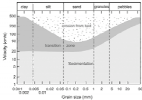
Figure 14b Velocity of fluids is an important factor in moving grains. Velocity can also affect river bottoms and cause erosion.
