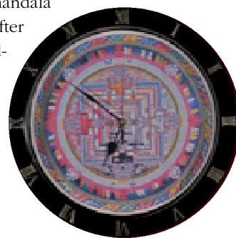
Figure 4. Colored grains of sand are used to make fantastic but ephemeral mandalas in Buddhist and other cultures.
