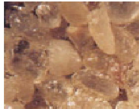
Figure 12. Immature sediment with angular fragments, mixture of sizes, various minerals, even mineral fragments.
